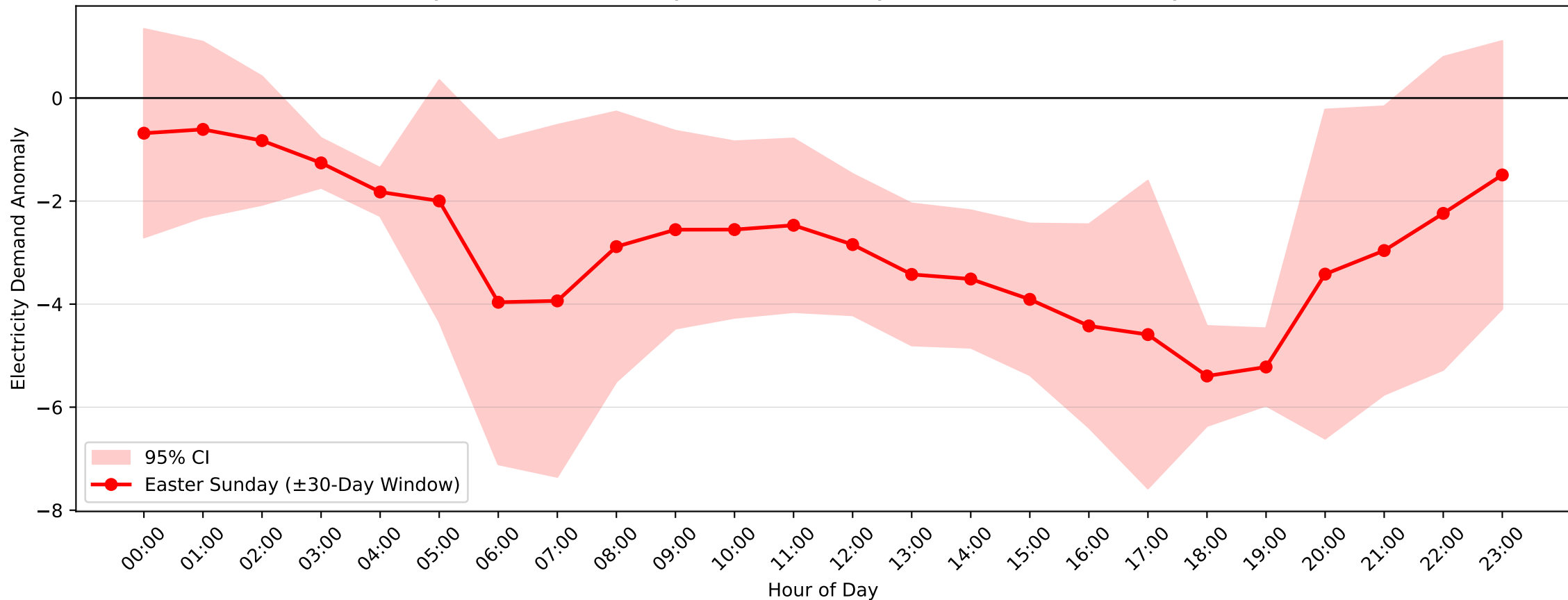
Revesby Demand Anomaly: Easter Sunday (2004–2017, \pm 30 -Day Window)
